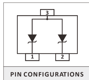
SOT-23 PACKAGE
